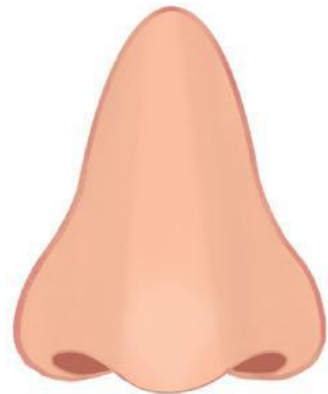
Nose (Mũi)
