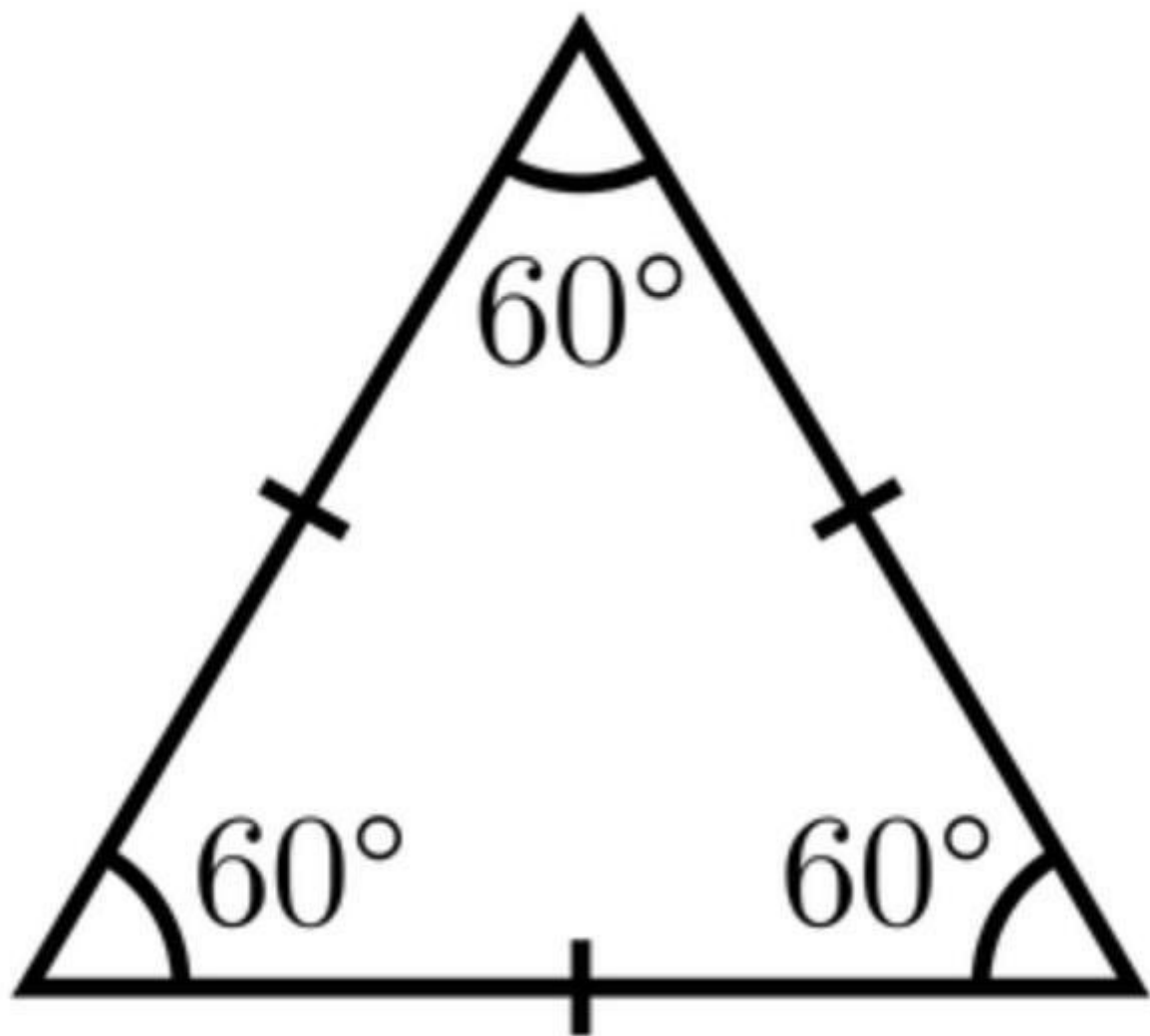
Equilateral triangle
