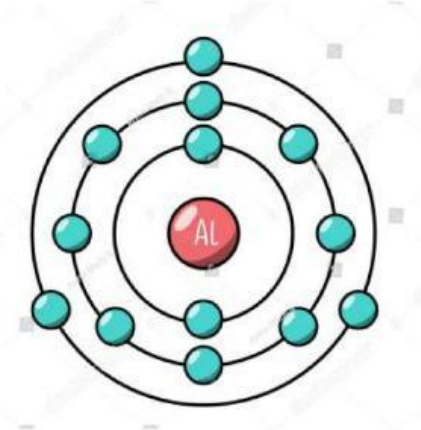
Gambar 2. Model Atom Bohr
