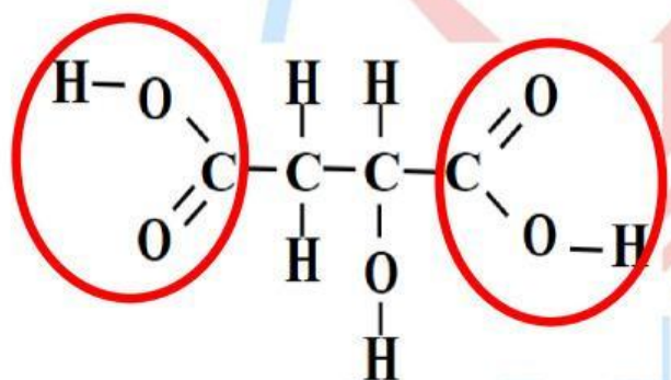
Malic acid
