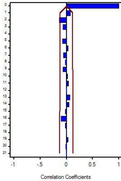
Autocorrelations
