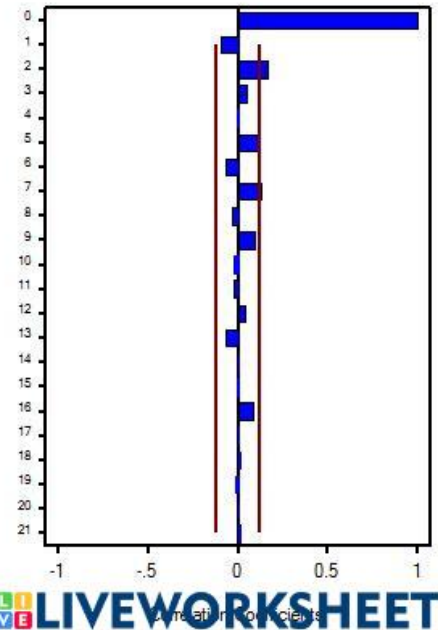
Inverse Autocorrelations
