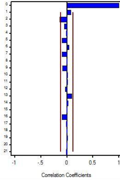
Partial Autocorrelations
