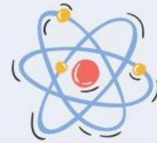
Rutherford
