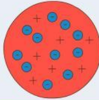
Thomson
