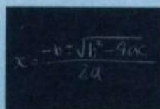
maths
