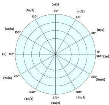
Graph A(3, 270^\circ)
