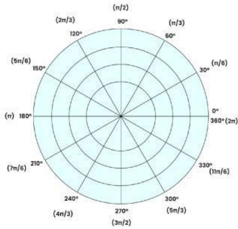
Graph A(3, 270^\circ)
