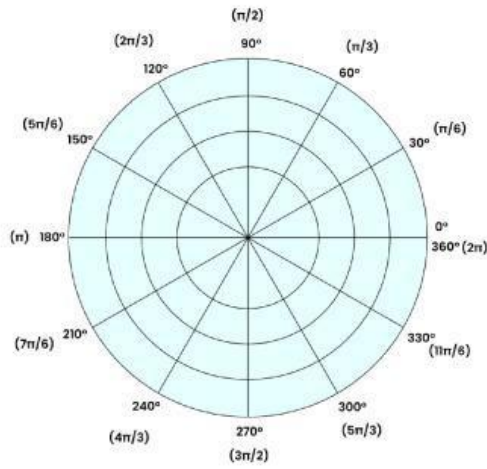
Graph \theta = 315^\circ
