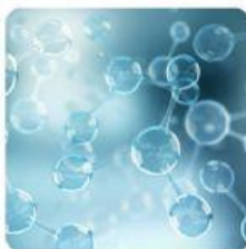
Great Oxygenation Event
