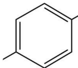
1-iodo-4-chlorobenzene
