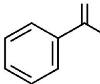
Benzoic acid
