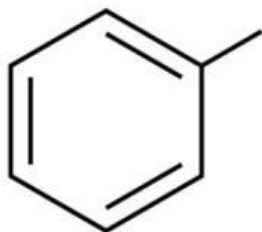
Toluene
