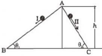
Fig. 6.1 \theta_1 < \theta_2
