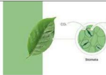
Stomata daun
