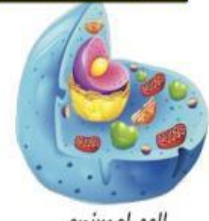
animal cell
