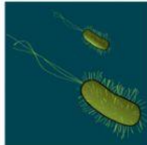
BACTERIS
