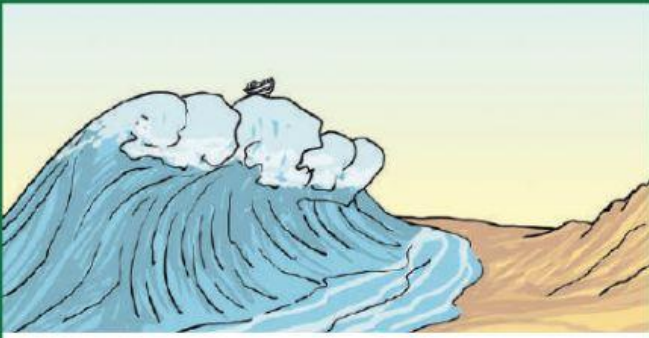
Tsunami
