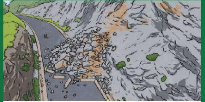
Landslide
