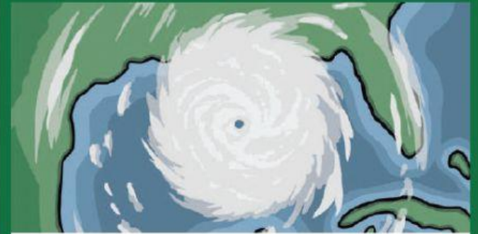
Hurricane
