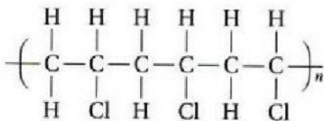
Polyvinyl chloride
