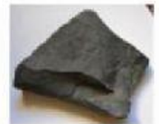
Shale
