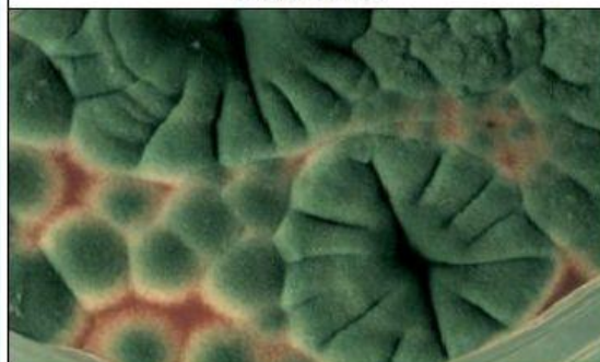
PENICILLIUM
