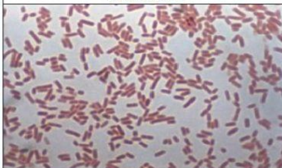
SALMONELLA
