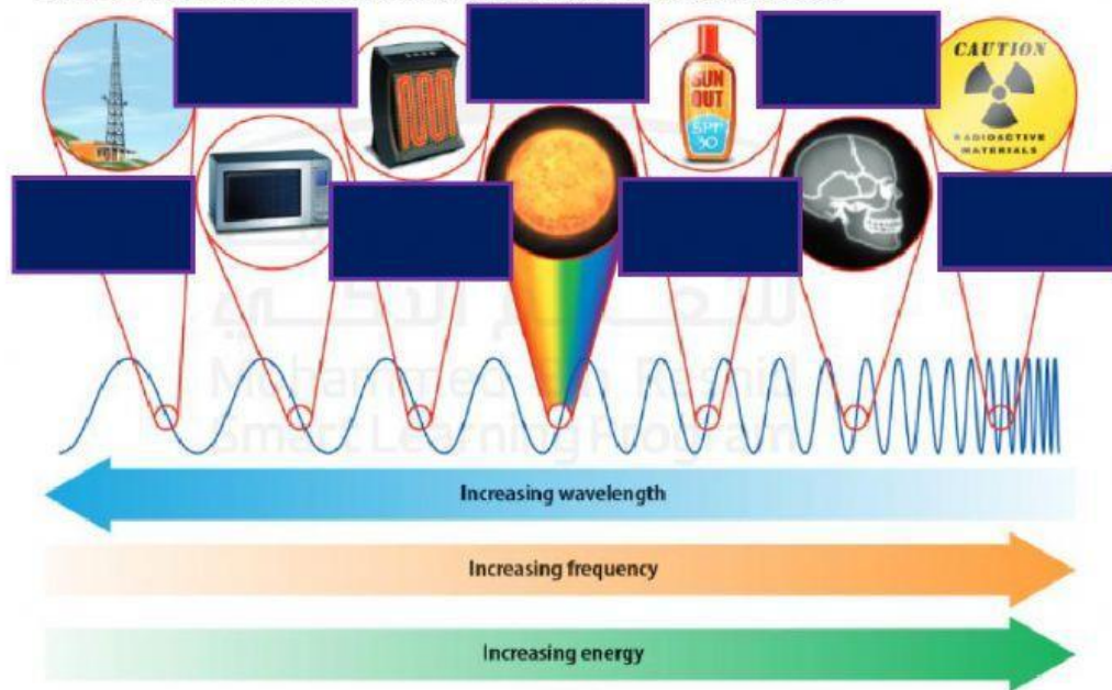
Figure 13 Electromagnetic waves have different wavelengths, frequencies, and energy.
