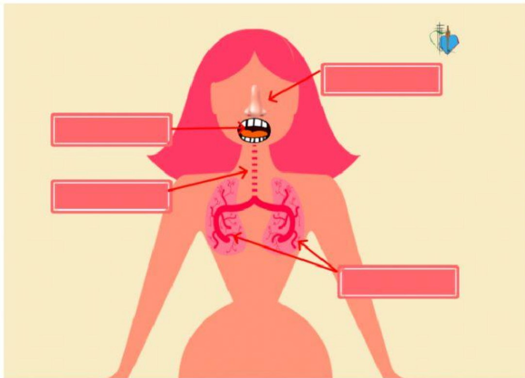
RESPIRATORY SYSTEM
