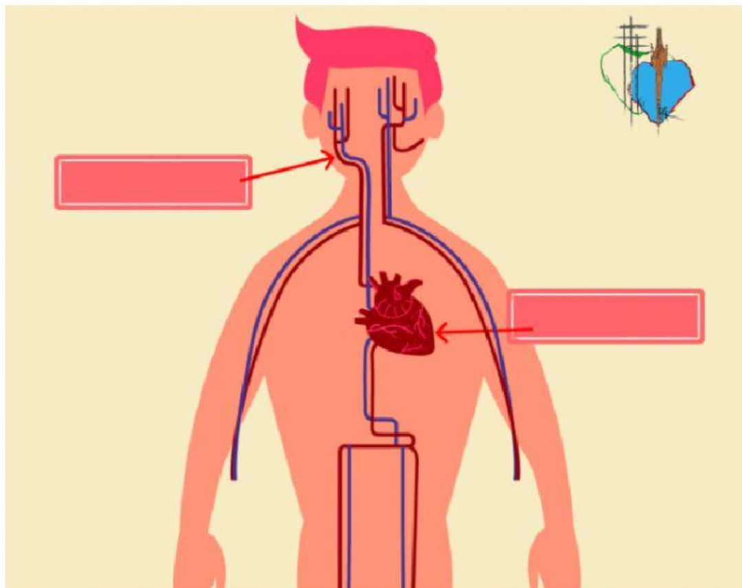
CIRCULATORY SYSTEM
