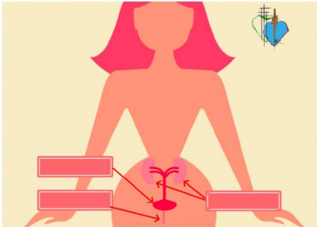
EXCRETORY SYSTEM
