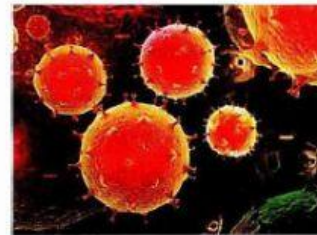
a virus
