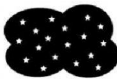
stars
