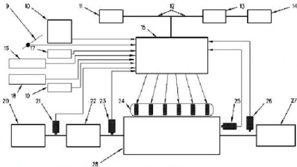
Illustration 2: Block Diagram of the Power Train Electronic Control System
