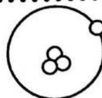
Hydrogen-3
