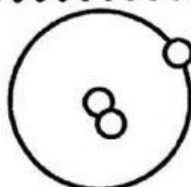
Hydrogen-2
