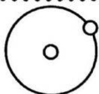
Hydrogen-1
