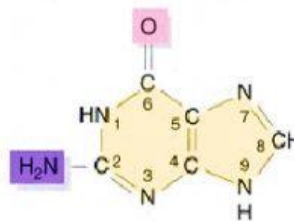
Guanine (G)
