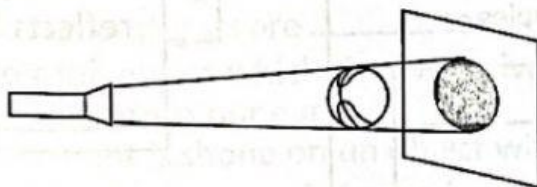
Object nearer to the screen
