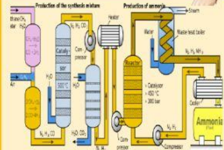
Gambar : Proses Haber Bosch www.png.download.id
