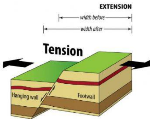
Normal fault
