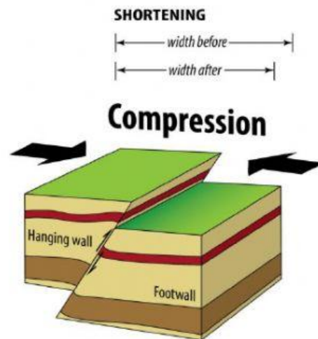
Reverse fault
