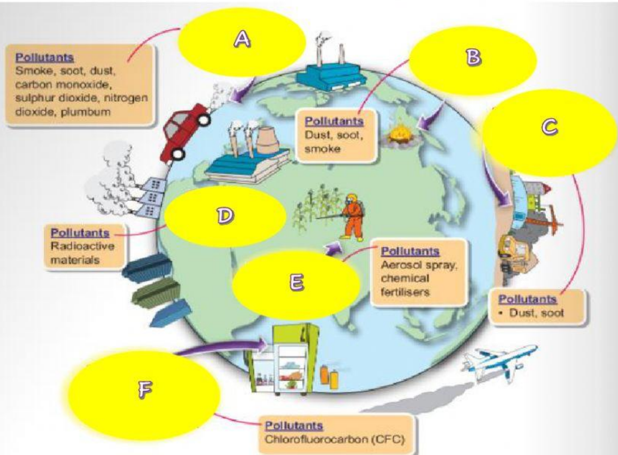
Figure 7.12 Sources of air pollutants
