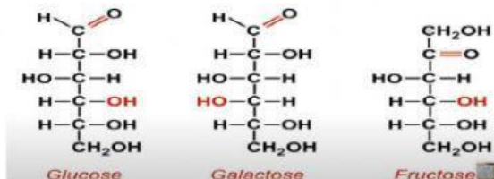
Carbohydrate Isomers
