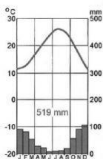
Klimogram 3.1
