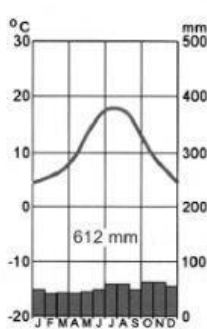
Klimogram 3.3
