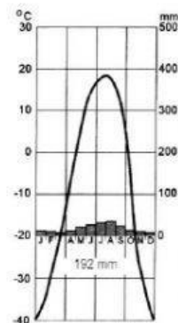
Klimogram 3.4
