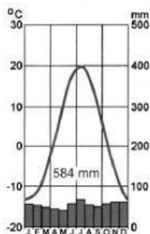
Klimogram 3.2
