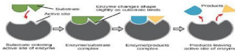
Gambar. 3 Teori Induksi Pas (model induced fit) Sumber: akkangyacob.blogspot.com
