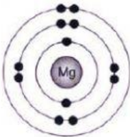
Atom magnesium (2.8.2) Magnesium atom (2.8.2)
