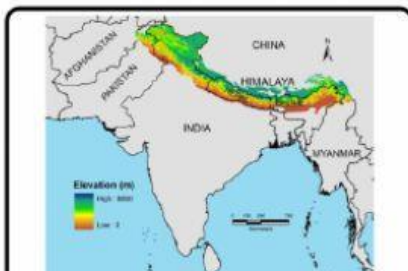
Himalayan mountains
