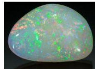
opal
