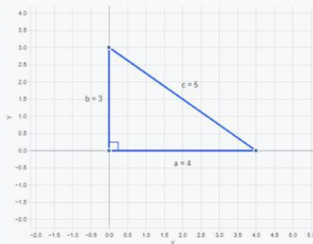
Pythagorean Theorem Geometry
