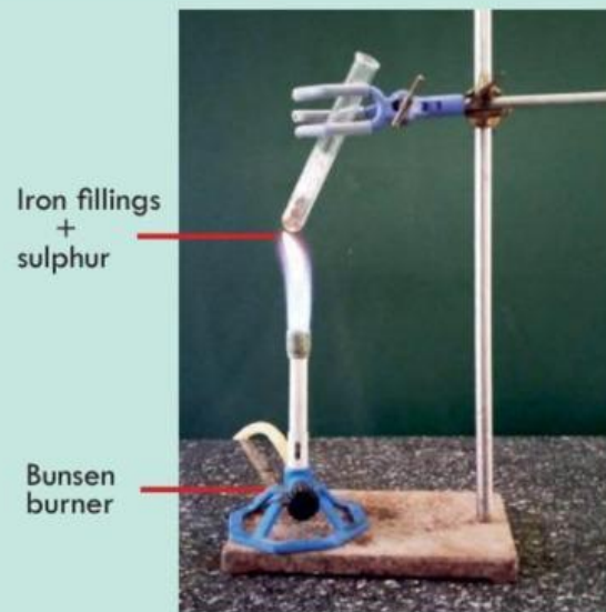
Figure 1.2 The reaction between iron and sulphur.
