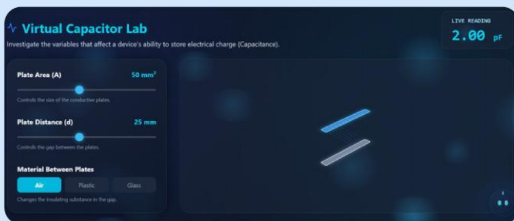
Fig 3. Virtual Capacitor Lab simulation view2
