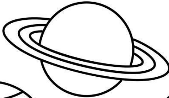
Saturn
