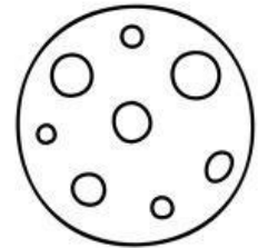
Mercury
