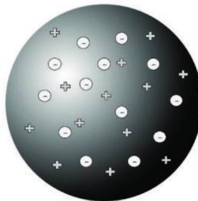
Thomson's Atomic Model
