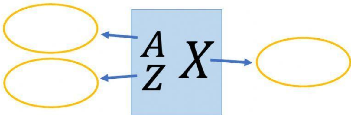
Gambar 1 – Lambang Atom
