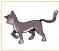
a cat
