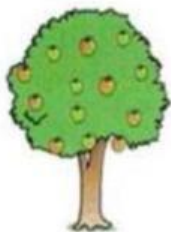
tree
