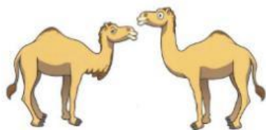
Camels
