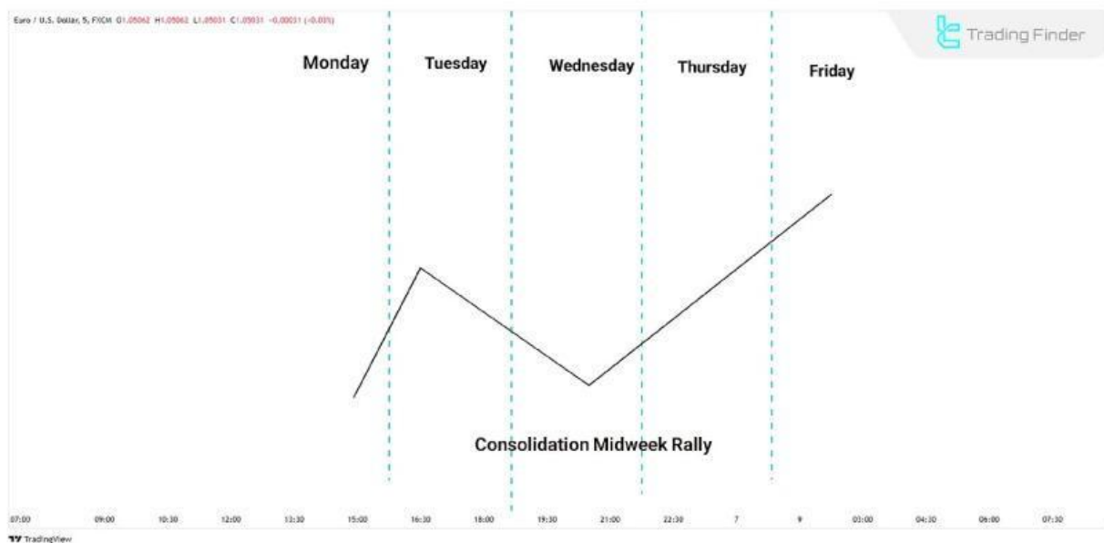
Schematic representation of the midweek bullish rally (Consolidation Midweek Rally) in ICT Weekly Profiles
