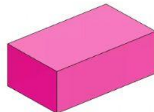
cuboid
