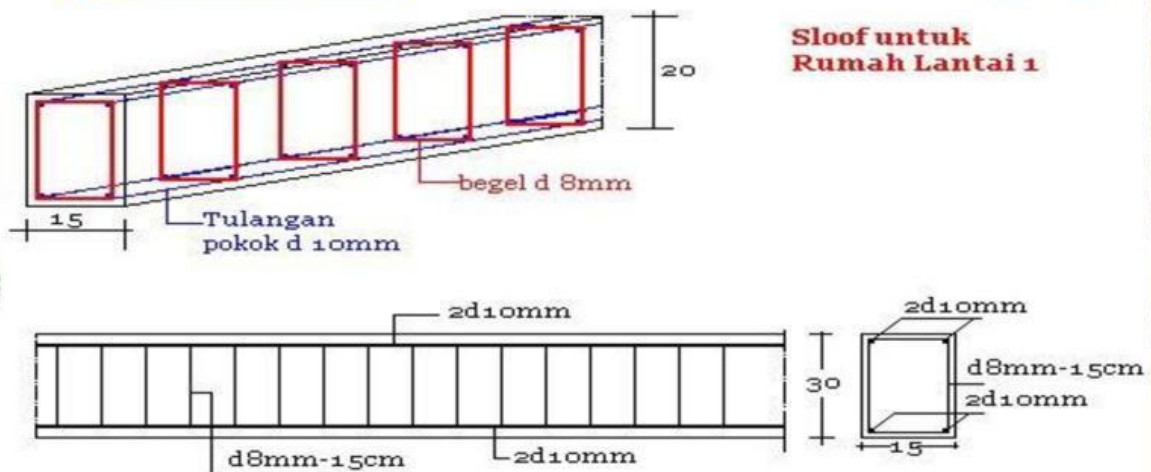
Gambar Sloof
