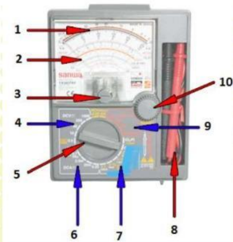
BAGIAN-BAGIAN MULTIMETER
