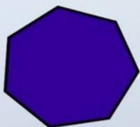
polygons
