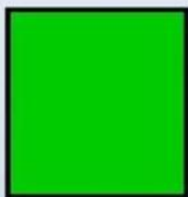
rectangles
