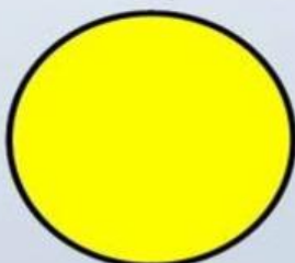
circles
