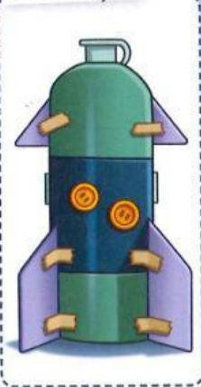
1 Galaxy 1
