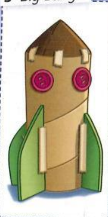
3 Big Bang 5
